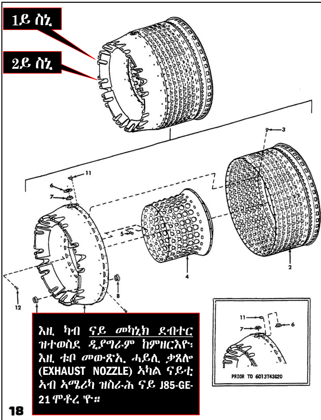
Figure 18. Combustion Liner Assembly
